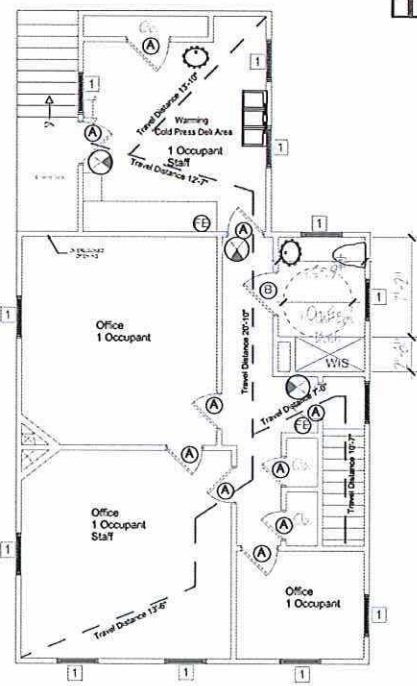
EXISTING DELI SECOND-STORY PLAN SCALE: 1/4" = 1' - 0"
