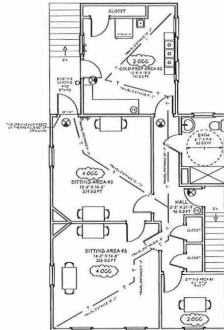
PROPOSED DELI 2ND-STORY PLAN
