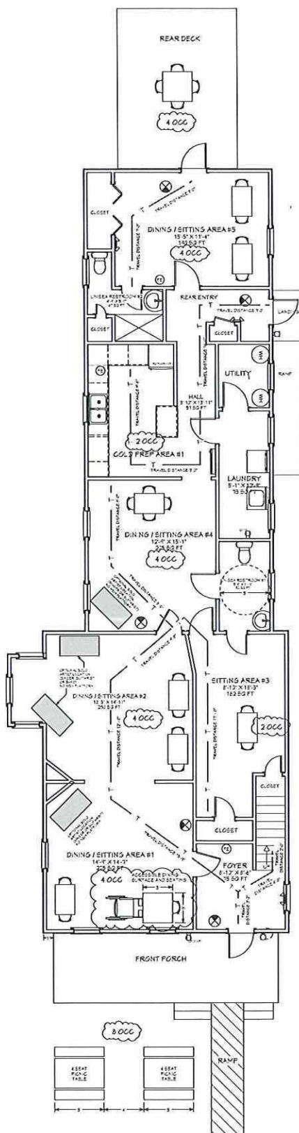
PROPOSED DELI 1ST-STORY PLAN SCALE: 1/4" = 1' - 0"
