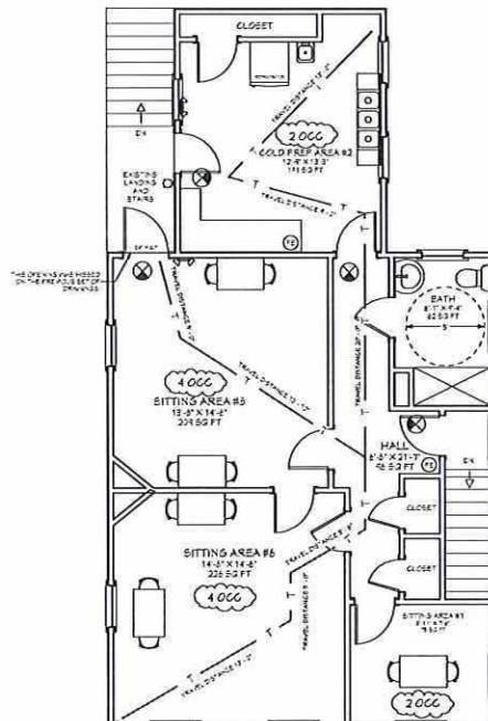
PROPOSED DELI 2ND-STORY PLAN SCALE: 1/4" = 1' - 0"
