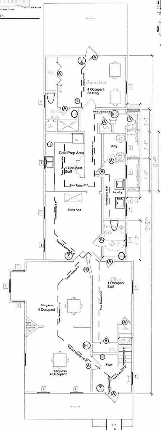
EXISTING DELI FIRST-STORY PLAN SCALE: 1/4" = 1' - 0"
